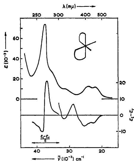
Figure 6. The absorption and circular dichroism spectra of (+)- cis -[Ru(phen) 2 (py) 2 ](ClO 4 ) 2 in water solution and the predicted absolute configuration.
